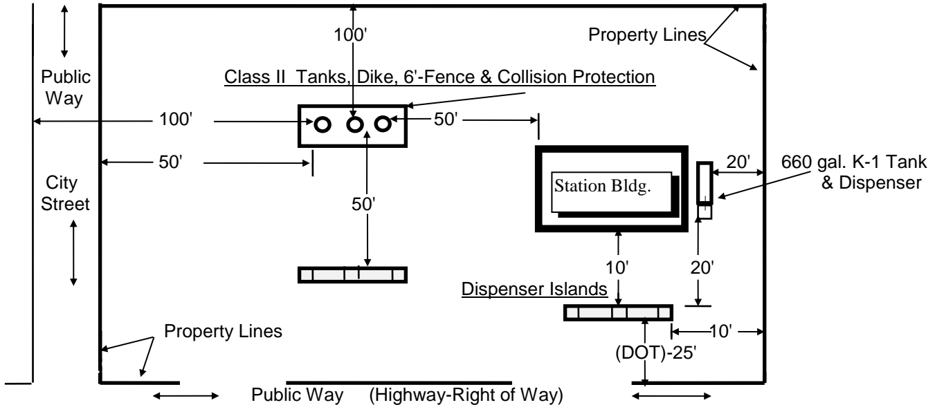
TYPICAL STORE LAYOUT
