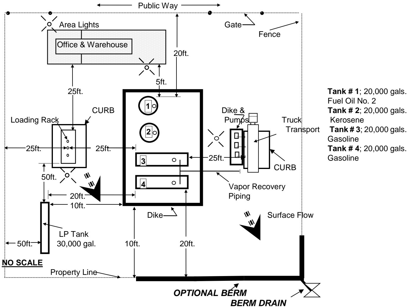
TYPICAL BULK PLANT INSTALLATION LAYOUT
